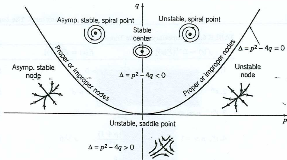
FIGURE 9.1.9 Stability diagram.
